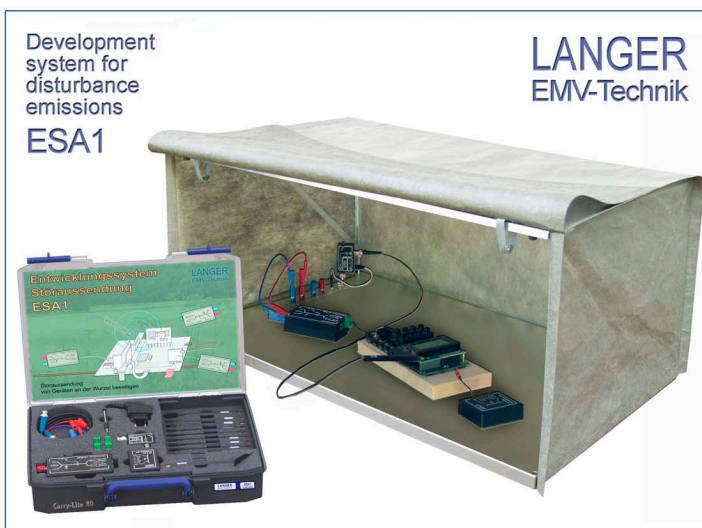
The ESA case contains all the equipment for the ESA workplace: GP21 base-plate, HFW21 RFtransformer, HFA21 RFcharge eliminator, shielding tent, near field probes and pre-amplifier
